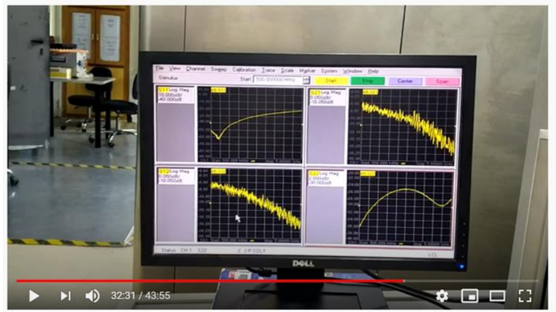
Lab Demo: Vector Network Analyzer VNA Calibration and Device Characterization
